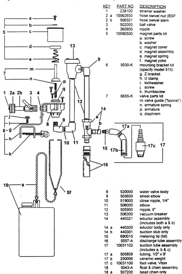
HydroMinder Model 515 Parts Diagram/List
